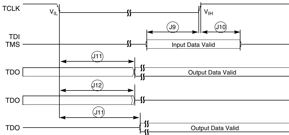
Figure 22. Test Access Port Timing
