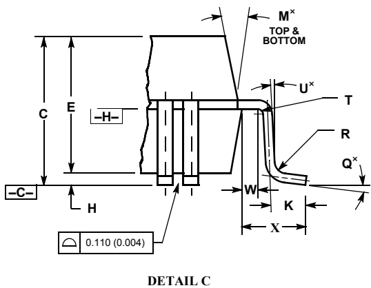
Case 864A-03 Figure 5. 160 QFP Package Dimensions
